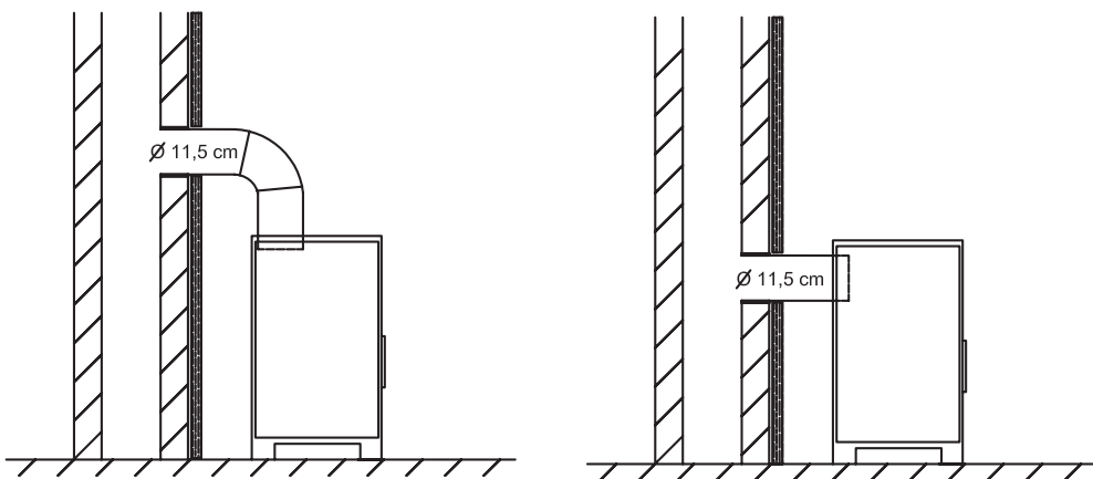
Drawing 16. Connecting the Sauna Stove to the Built-in Chimney
