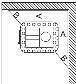
Drawing 15. Safe Distances (in cm)
